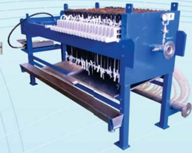
Chamber Filter Press
